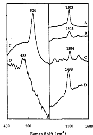
Figure 1. Resonance Raman spectra of (A) BIDPhE, (B) [Zn(BIDPhE)Cl 2 ], (C) [Fe 2 O(XDK)(BIDPhE) 2 (NO 3 ) 2 ] dissolved in CH 2 Cl 2 , and (D) wild type ribonucleotide reductase R2 protein from E. coli , strain N6405/PSPS2, dissolved in Tris buffer, pH 7.6, 5% glycerol. All spectra were recorded at room temperature with Kr ion laser excitation at 406.7 nm.
