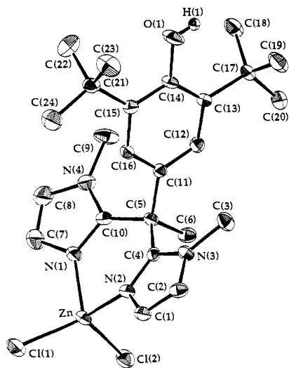
Figure 2. ORTEP diagram of [\text{Zn}(\text{BIDPhE-H})\text{Cl}_2]\cdot\text{CH}_3\text{CN} showing the 50% probability thermal ellipsoids. Selected interatomic distances (Å) and angles (deg) are as follows: Zn–Cl1, 2.224(1); Zn–Cl2, 2.237(1); Zn–N1, 2.003(3); Zn–N2, 2.012(3); Cl1–Zn–Cl2, 120.19(4); Cl1–Zn–N1, 113.4(1); Cl1–Zn–N2, 112.57(9); N1–Zn–N2, 89.4(1).
